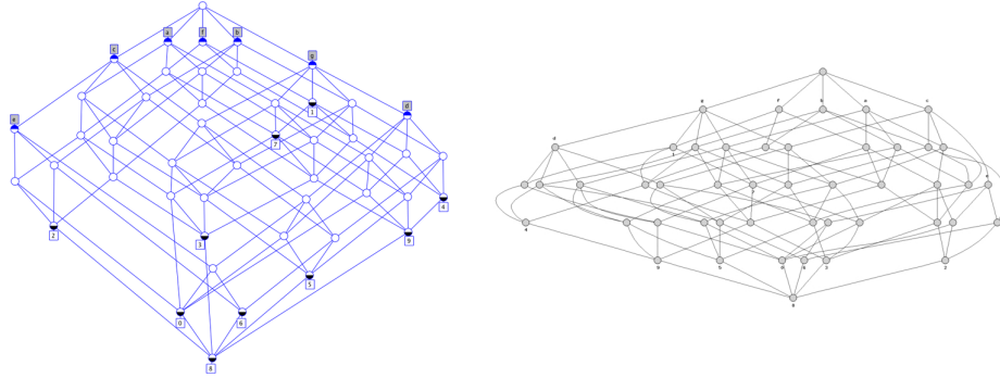
Fig. 3. The “digits” example: Wille’s layout, Graphviz
