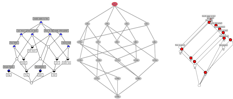
Fig. 8. The “live in water” example: ConExp, Galicia, Siena
