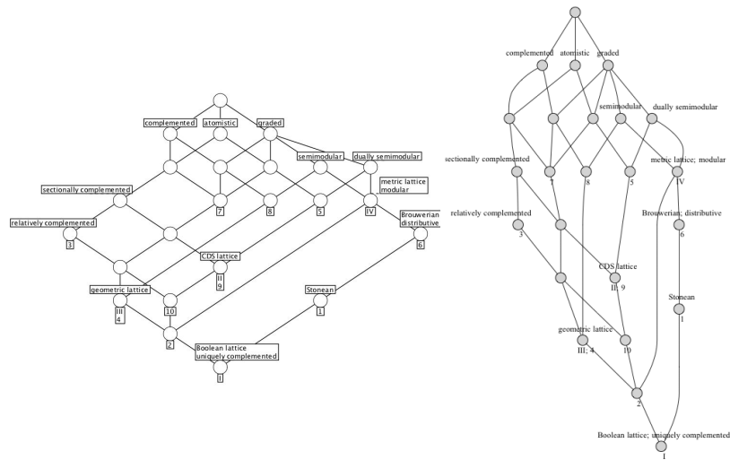
Fig. 7. The “lattice properties” example: Wille’s layout, Graphviz
