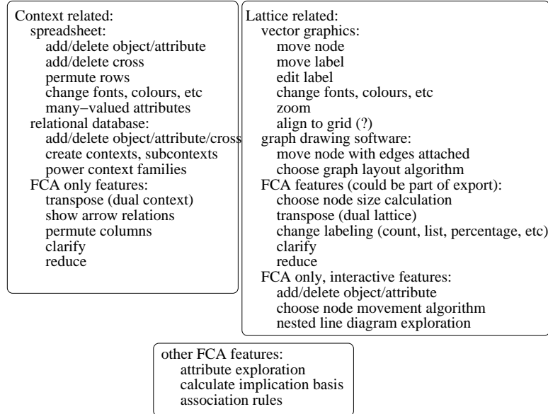
Fig. 1. Tasks for FCA software
