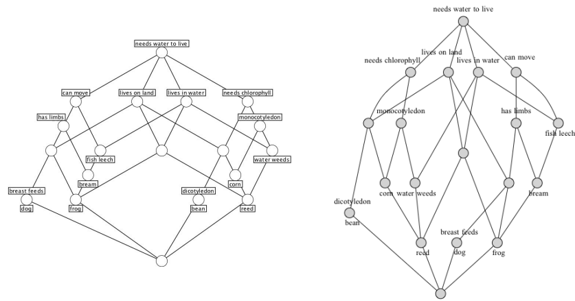
Fig. 9. The “live in water” example: Wille’s layout, Graphviz
